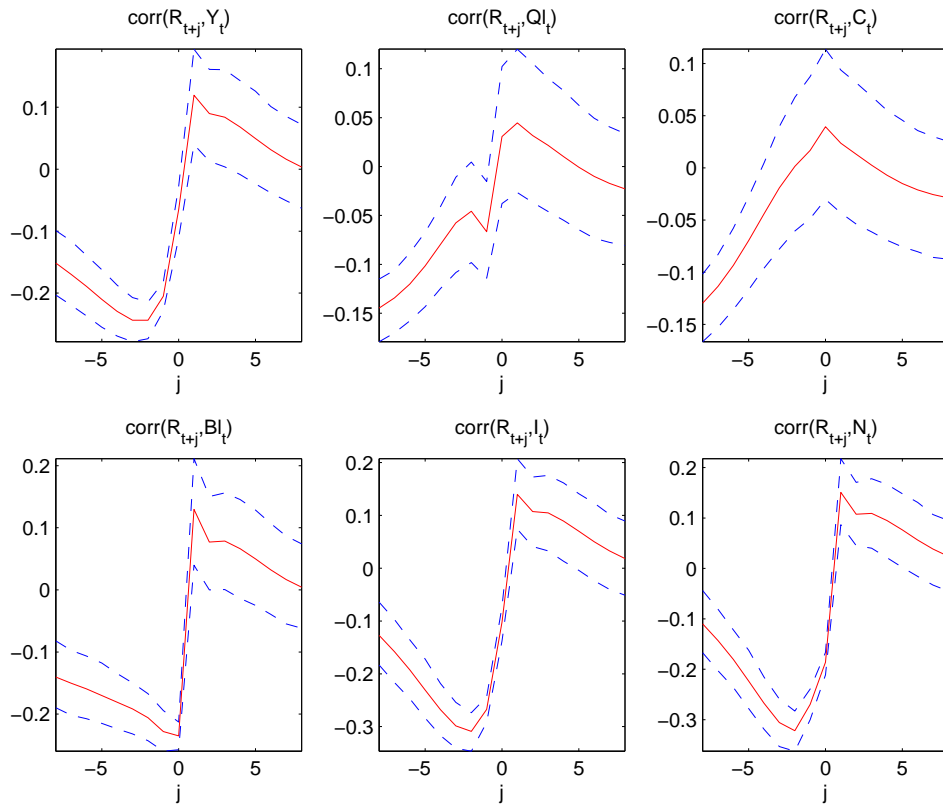
Figure 6: Theoretical dynamic correlations from indeterminate model with redistribution shock
