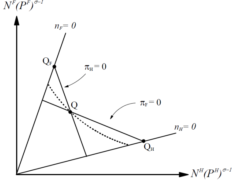
Figure 1: Optimal NTA
