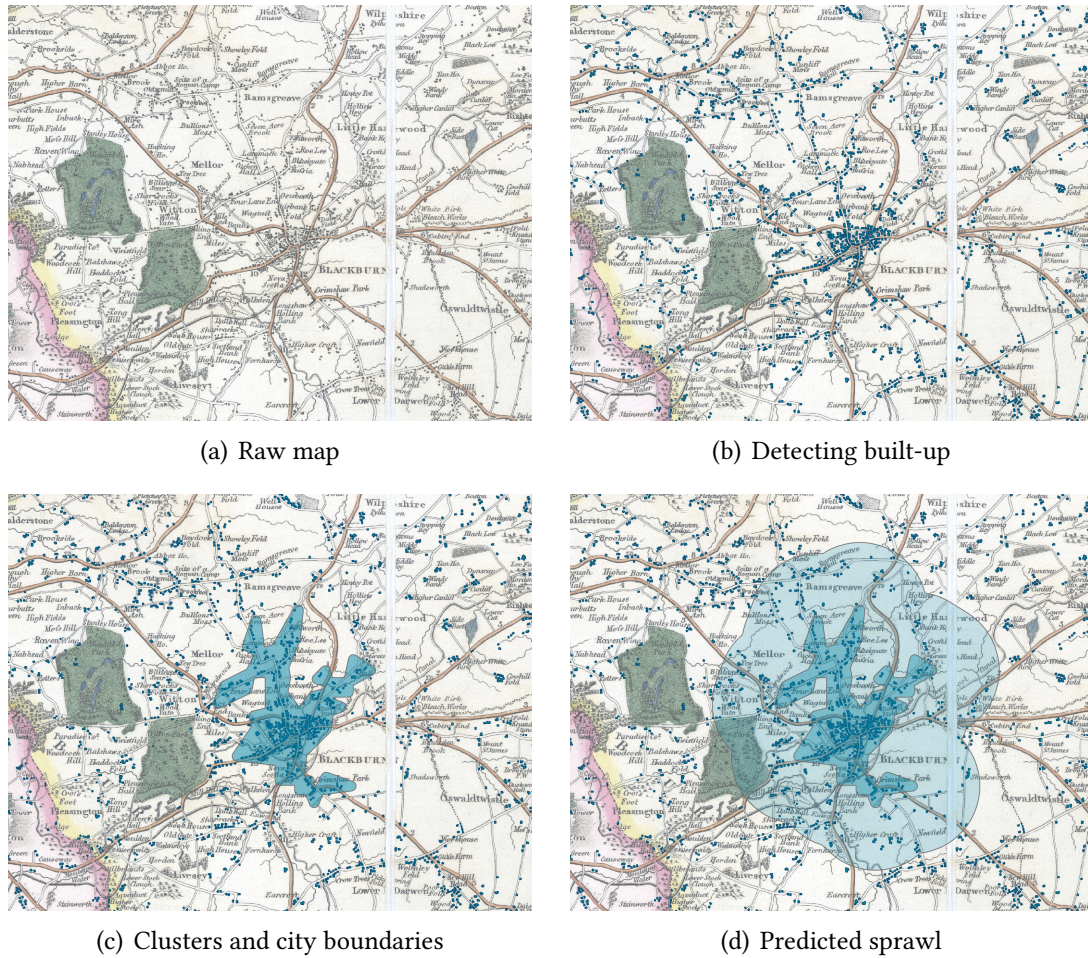
Figure 6. Clustering procedure.
