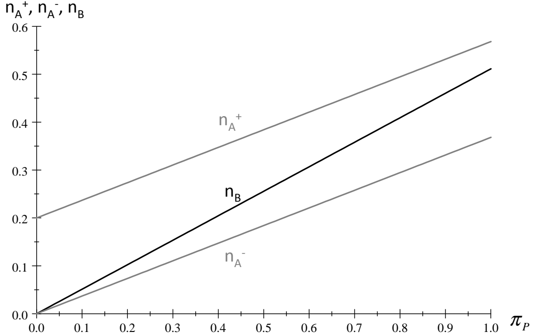
Figure 2: Investment as function of beliefs
