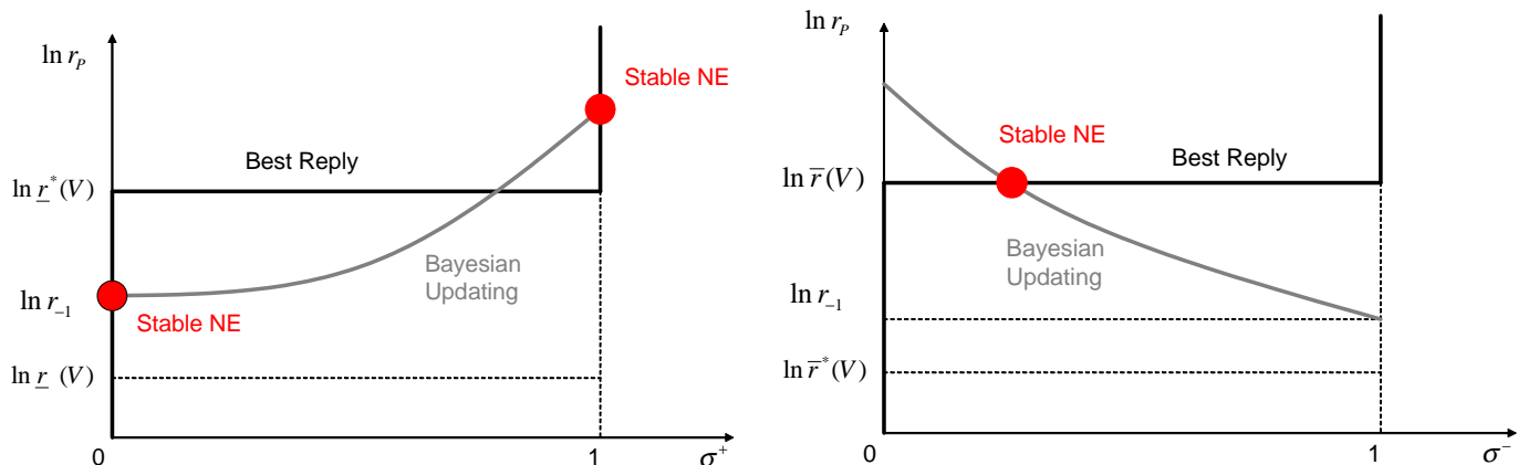
Figure 9: Multiple PBE and Mixed-Strategy PBE
