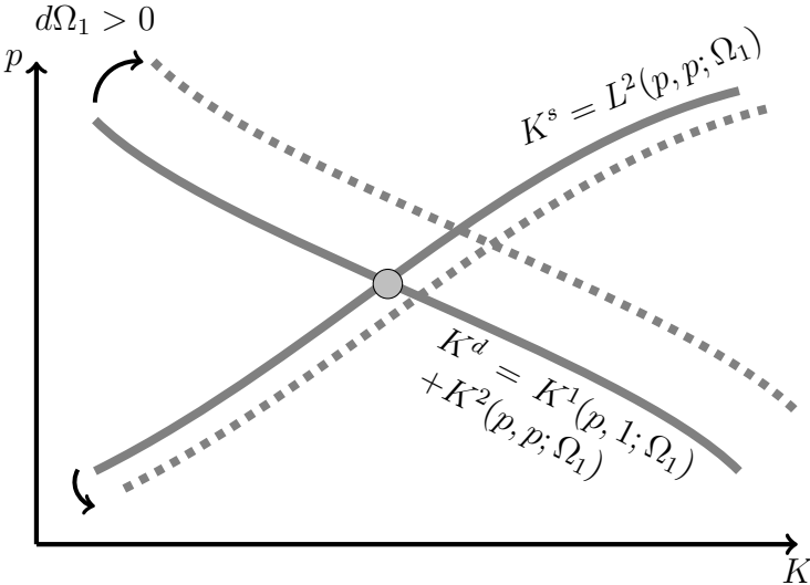
Figure 5: Illustration of the Sufficient Conditions of Proposition 3
